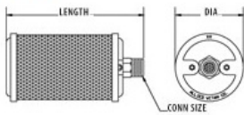
Single Chamber-Male 1/8"- 2"
